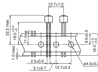
●B-06-RTF-25
