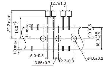
●B-02-RT • RTF/B-03-RT
