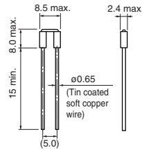
●B-03-R Series
