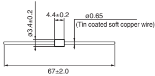
●B-01-A Series
