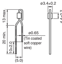
●B-01-R Series
