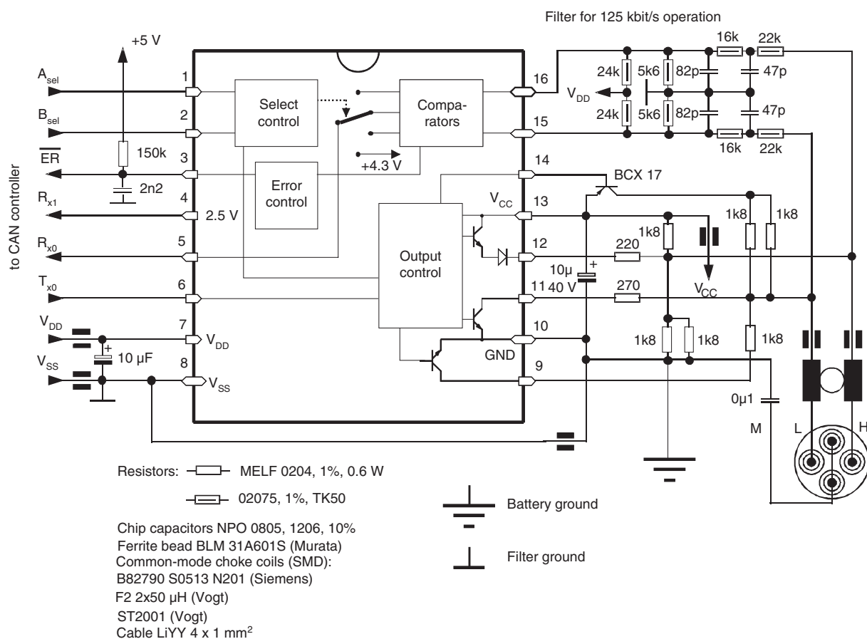
Figure 6-2. Application Circuit
