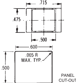
J53 Rocker Style
