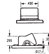
J53 Rocker Style
