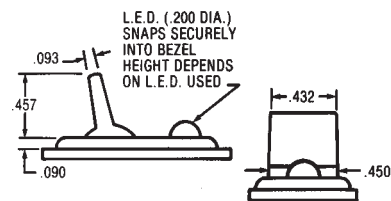
J60 Paddle Style w/Bezel for L.E.D.
