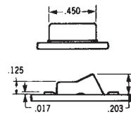
J50 Rocker Style
