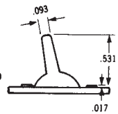
J60 Paddle Style
