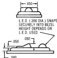
J50 Rocker Style w/Bezel for L.E.D.
