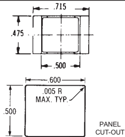
J50 Rocker Style
