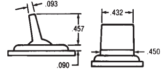
J60 Paddle Style w/Bezel
