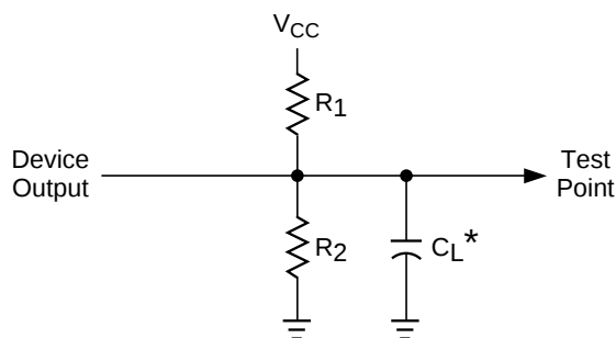
Figure 2. Test Load
