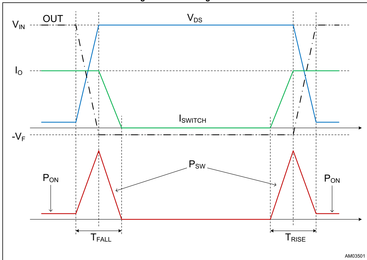
Figure 14. Switching losses
