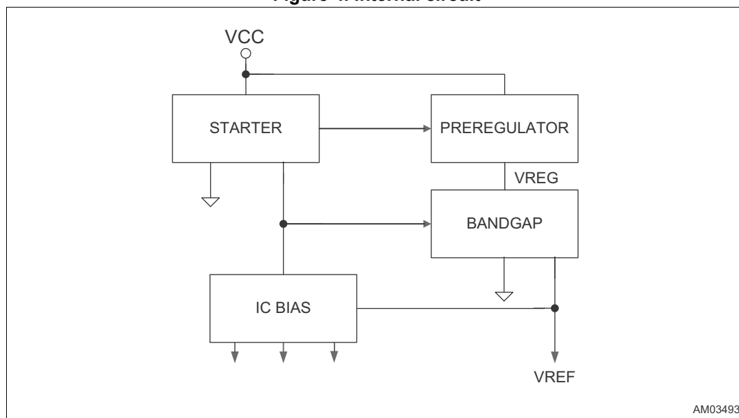
Figure 4. Internal circuit
