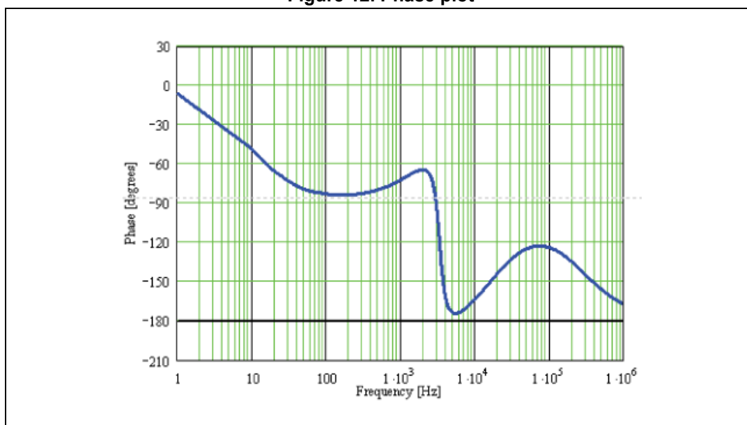
Figure 12. Phase plot
