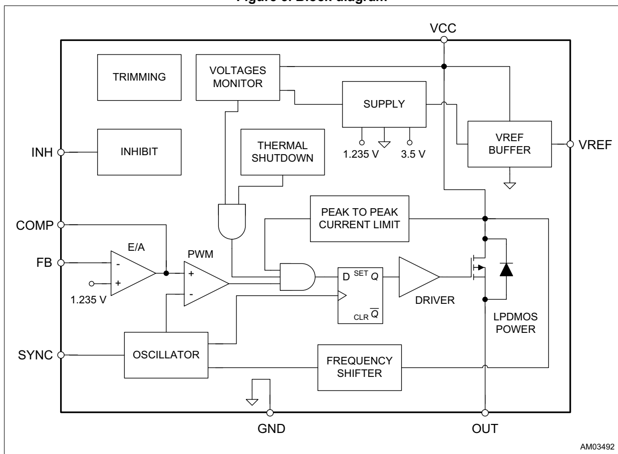
Figure 3. Block diagram
