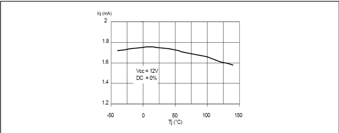
Figure 31. Quiescent current vs. junction temperature
