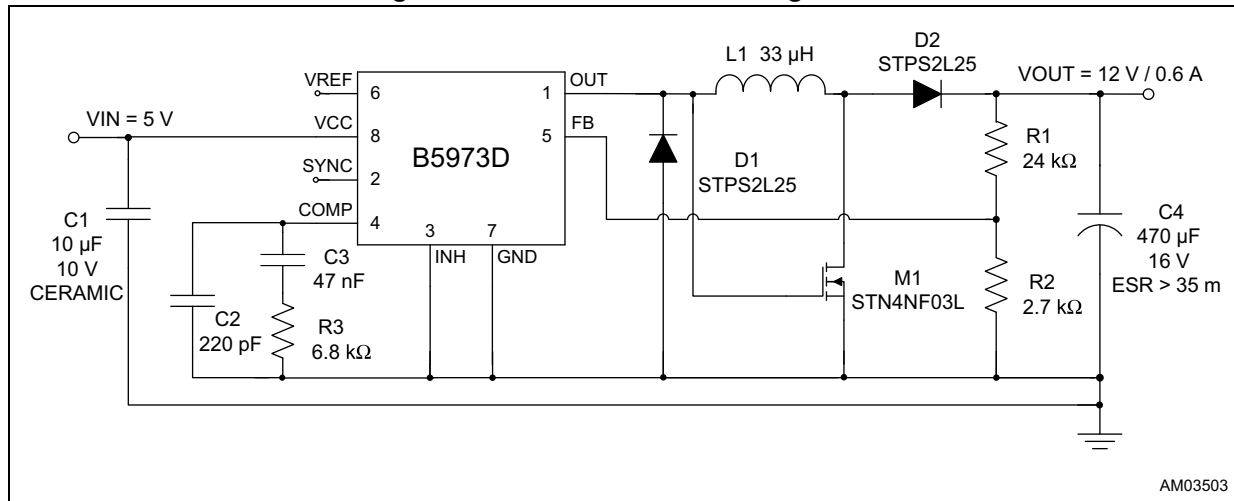
Figure 22. Positive buck-boost regulator
