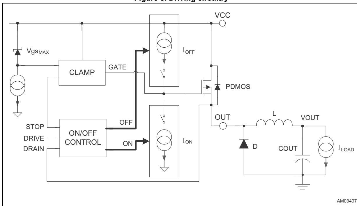
Figure 8. Driving circuitry
