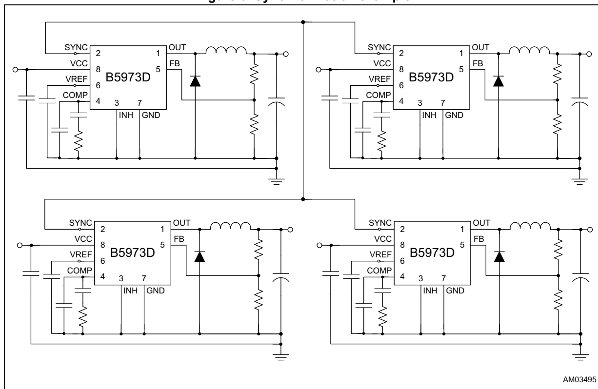
Figure 6. Synchronization example
