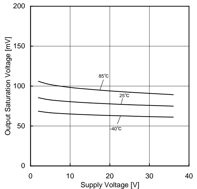
Figure 5. Output Saturation Voltage vs Supply Voltage ( I_{OL}=4\text{mA} )
