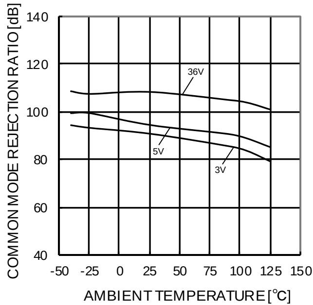
Figure 72. Common Mode Rejection Ratio - Ambient Temperature
