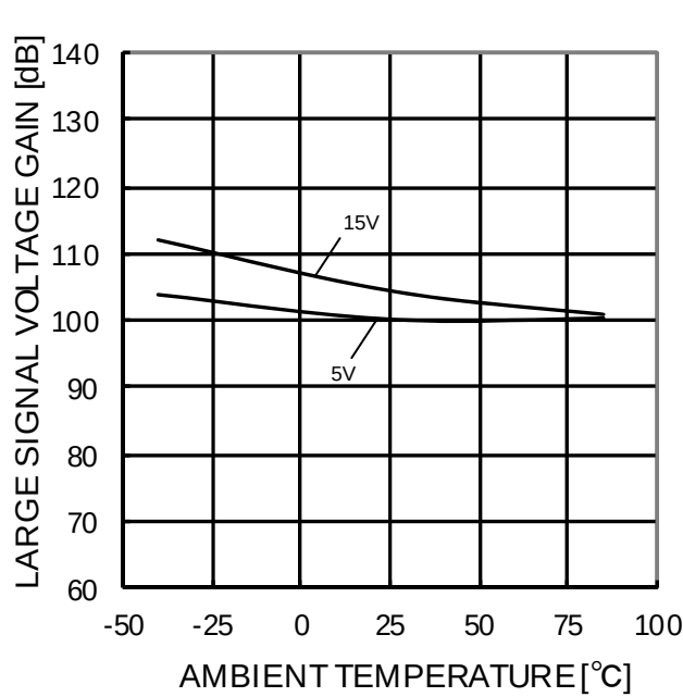
Figure 46. Large Signal Voltage Gain - Ambient Temperature (RL=2kΩ)
