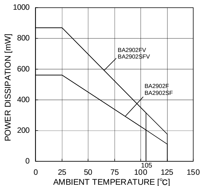
Figure 74. Derating Curve
