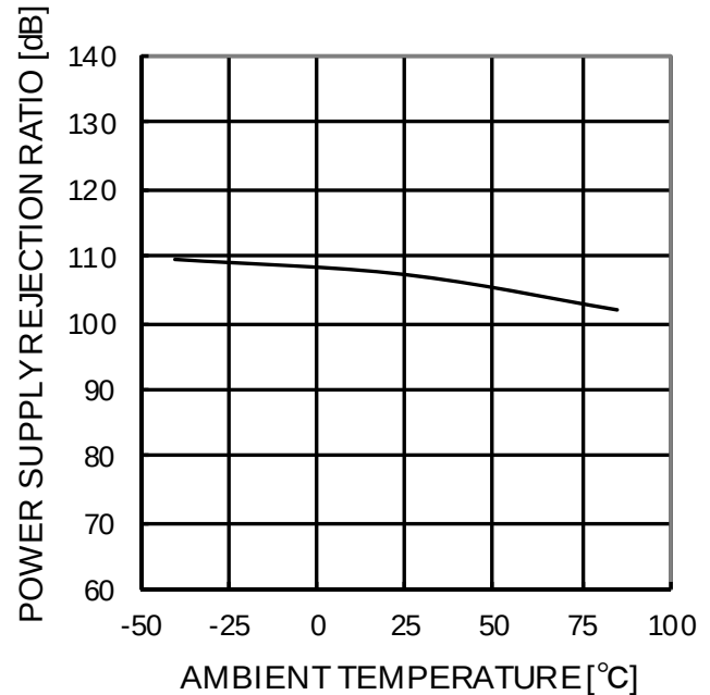
Figure 49. Power Supply Rejection Ratio - Ambient Temperature
