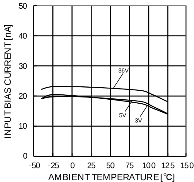
Figure 64. Input Bias Current - Ambient Temperature ( V_{ICM}=0V , OUT=1.4V )
