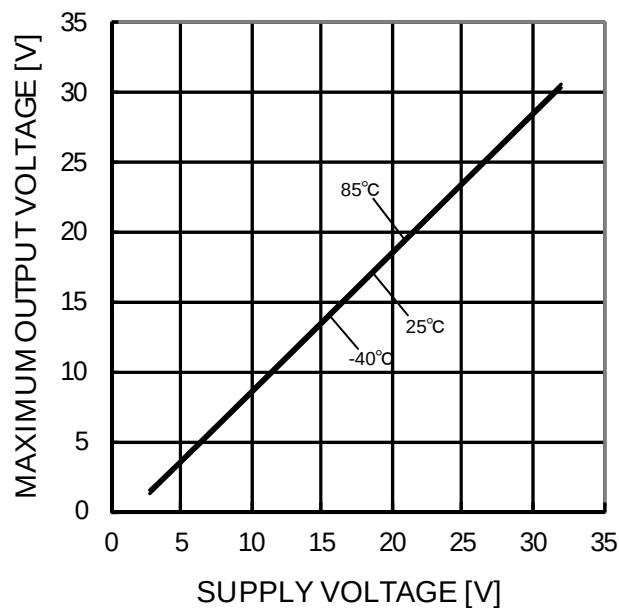
Figure 29. Maximum Output Voltage - Supply Voltage (RL=10kΩ)
