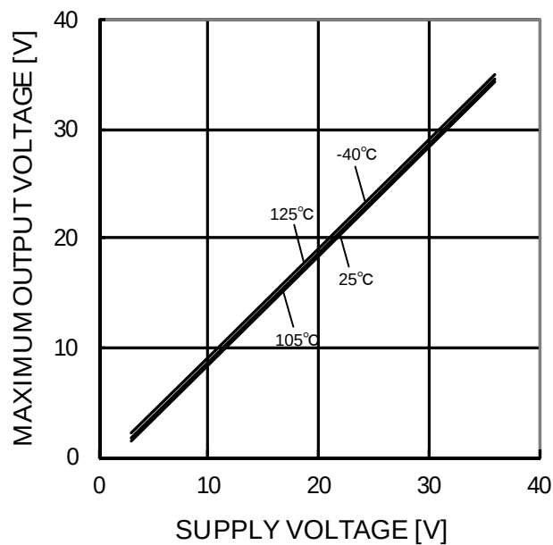
Figure 77. Maximum Output Voltage - Supply Voltage ( R_L=10k\Omega )
