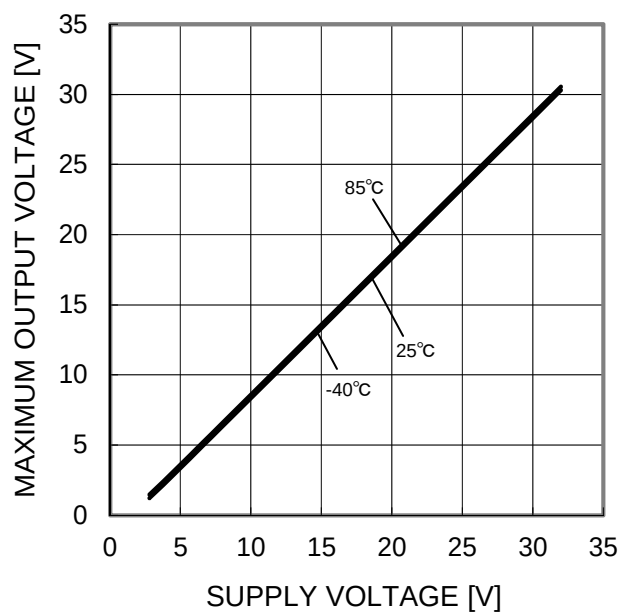
Figure 5. Maximum Output Voltage - Supply Voltage ( R_L=10k\Omega )
