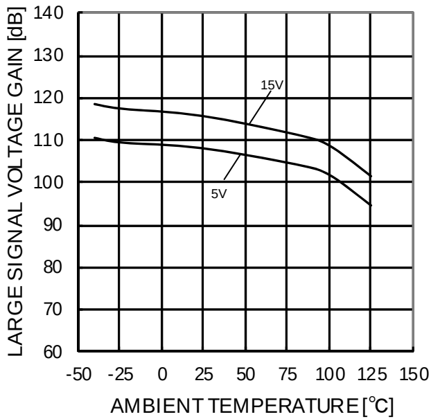
Figure 94. Large Signal Voltage Gain - Ambient Temperature ( R_L=2k\Omega )
