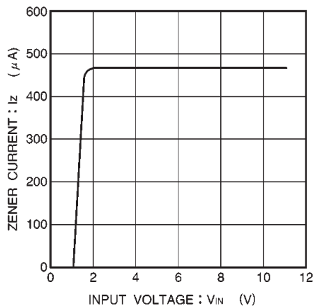
Fig.6 Zener current vs. input voltage
