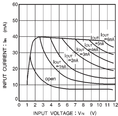
Fig.9 Input current vs. input voltage
