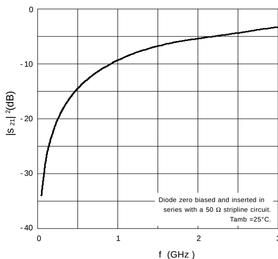
Fig.4 Isolation ( |S_{21}|^2 ) of the diode in off-state as a function of frequency; typical values.
