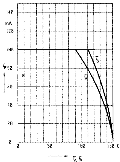
Forward current I_F = f(T_A, T_S)
