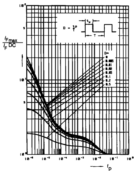
Permissible load I_{Fmax} / I_{FDC} = f(t_p)
