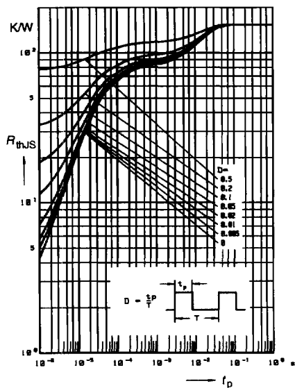
Permissible load R_{thJS} = f(t_p)
