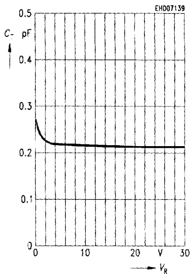
Diode capacitance C_T = f(V_R) f = 1 \text{ MHz}
