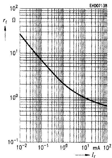
Forward resistance r_f = f(I_F) f = 100 \text{ MHz}
