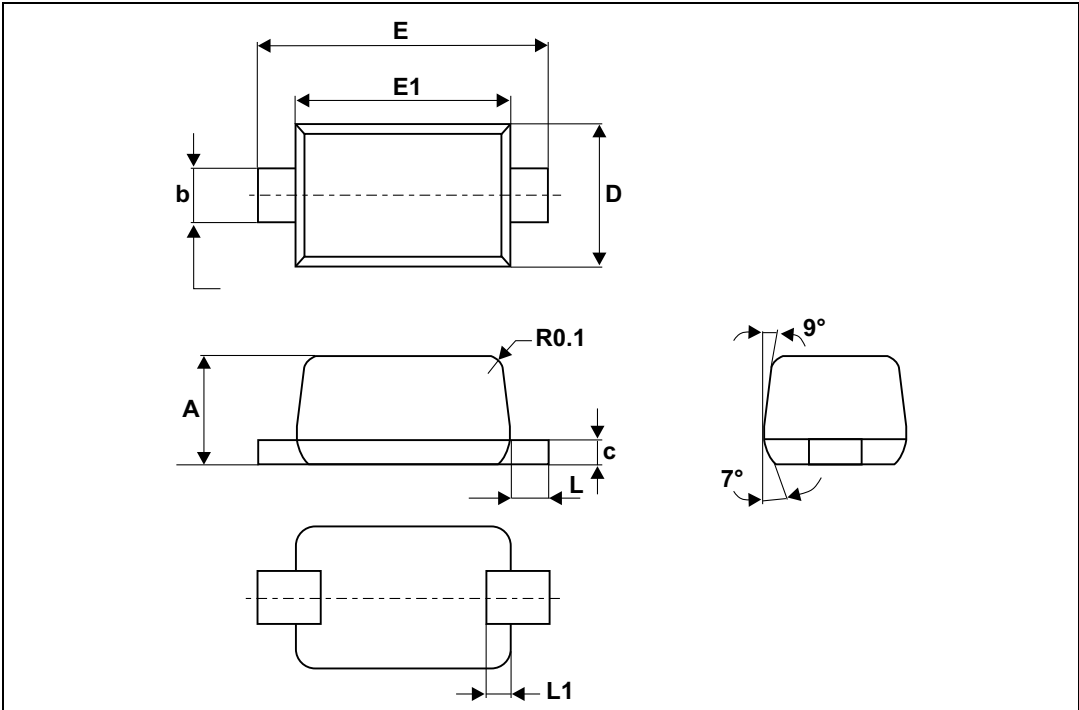
Figure 16. SOD-523 dimension definitions
