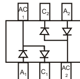
BAT54SDW* Marking: KL8
