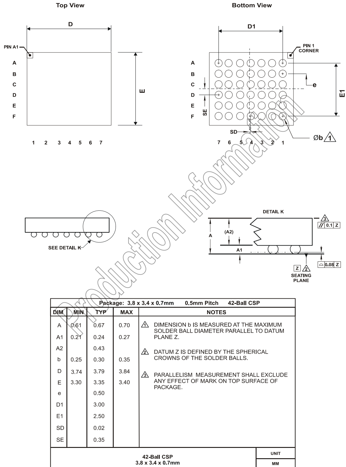
Figure 11.1: BlueCore3-ROM CSP Package Dimensions
