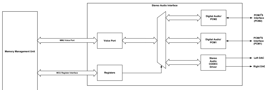
Figure 9.1: Audio Interface
