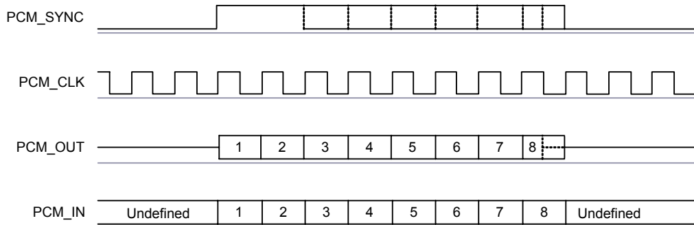
Figure 9.5: Long Frame Sync (Shown with 8-bit Companded Sample)
