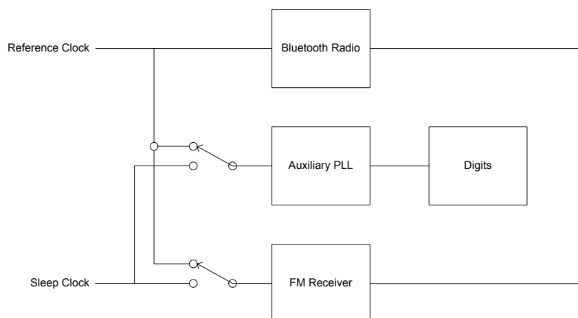
Figure 6.1: Clock Architecture
