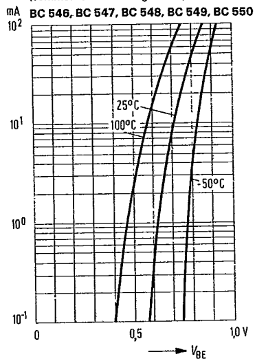
Collector current I_{\text{C}} = f(V_{\text{BE}}) V_{\text{CE}} = 5 \text{ V} (common-emitter configuration)
