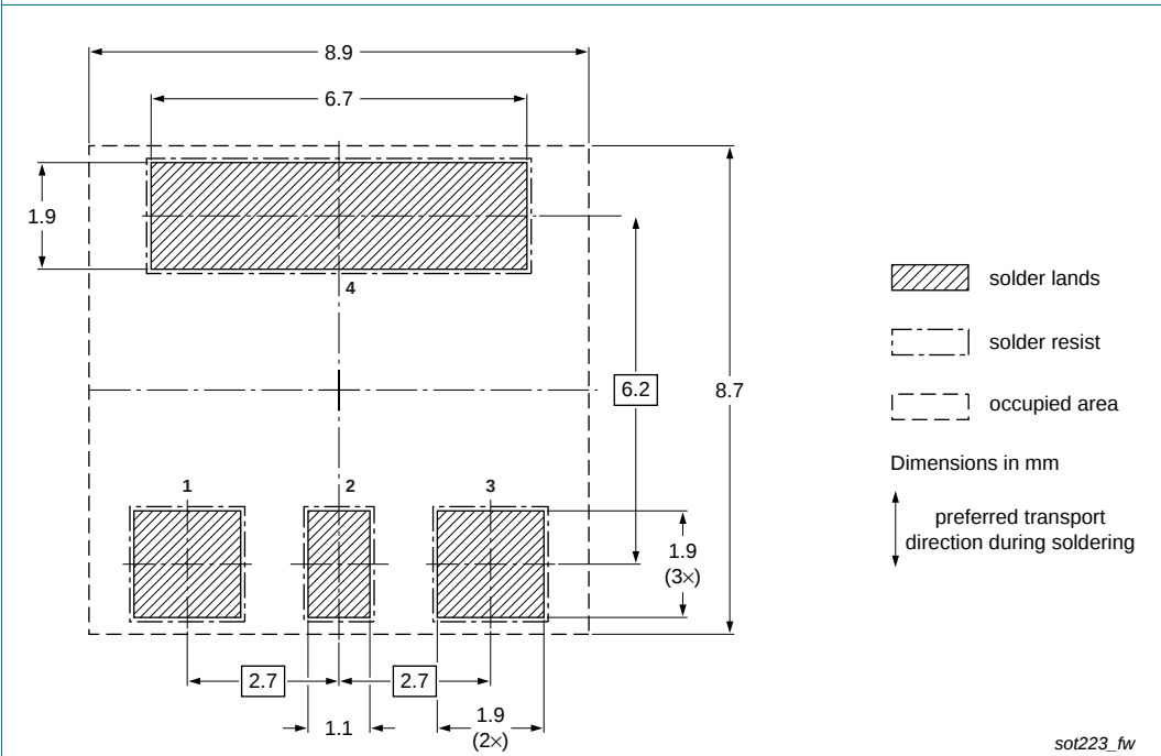
Fig 27. Wave soldering footprint SOT223 (SC-73)
