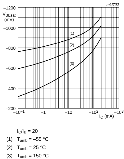
Fig 13. TR2 (PNP): Base-emitter saturation voltage as a function of collector current; typical values
