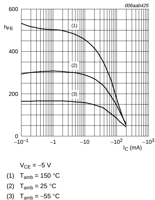
Fig 10. TR2 (PNP): DC current gain as a function of collector current; typical values
