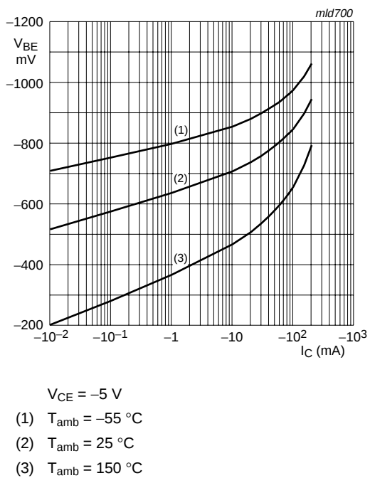
Fig 12. TR2 (PNP): Base-emitter voltage as a function of collector current; typical values
