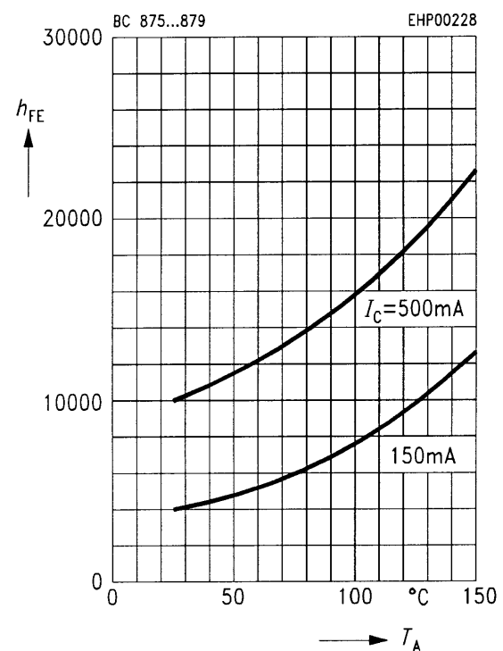
DC current gain h_{\text{FE}} = f(T_A)
