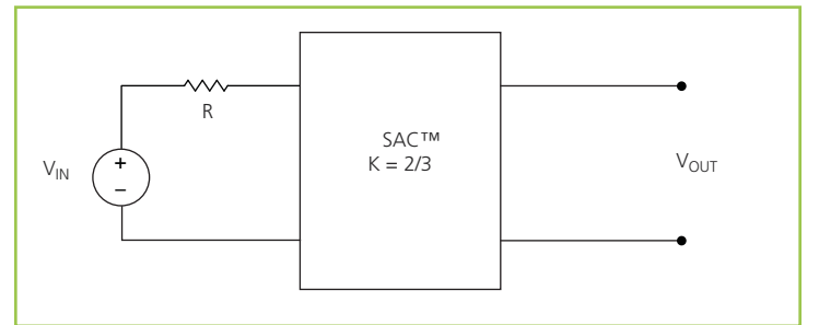
Figure 14 — K = 2/3 Sine Amplitude Converter™ with series input resistor
