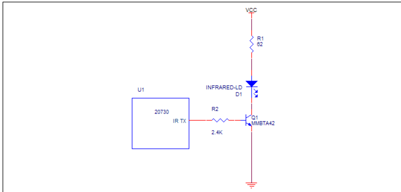
Figure 2. Infrared TX
