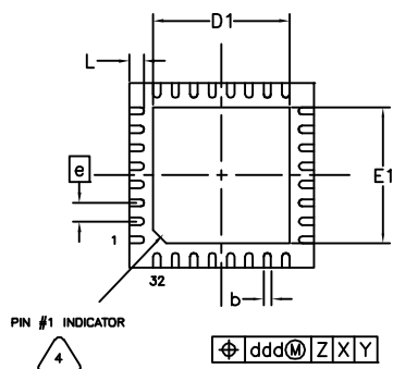
BOTTOM VIEW (32 LEADS)
