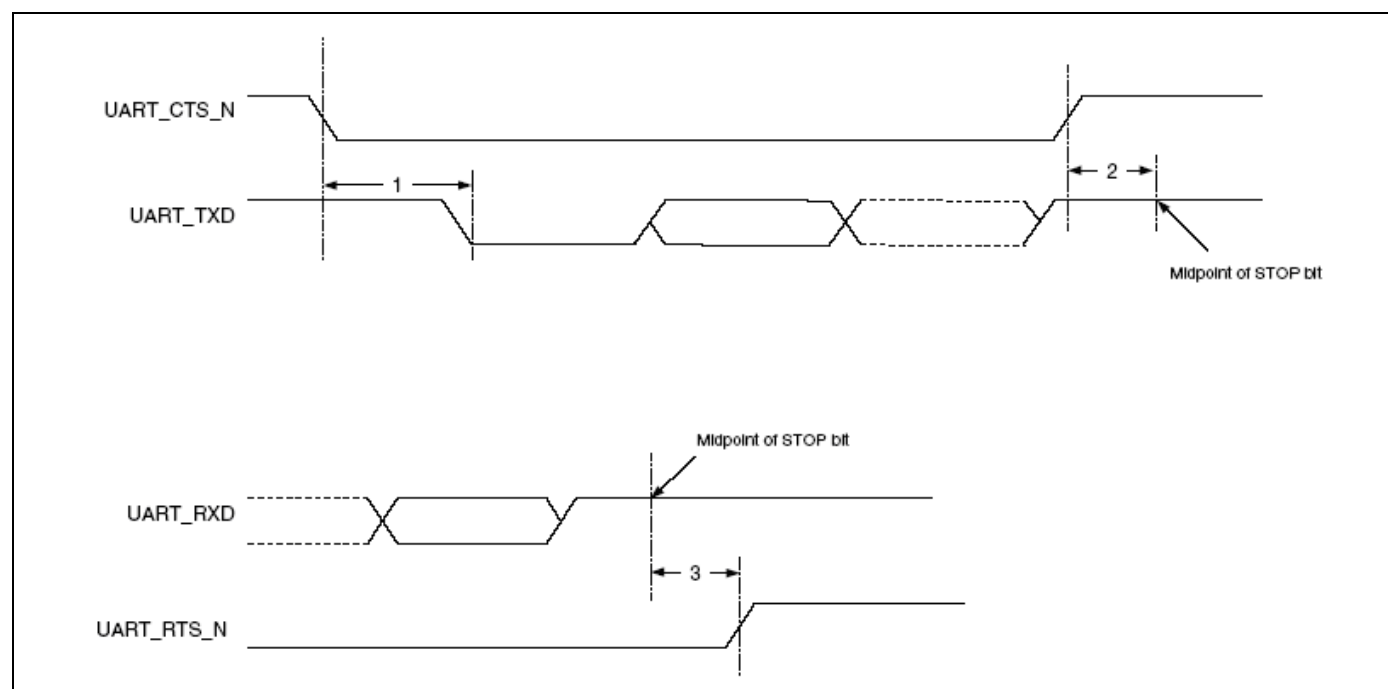
Figure 12. UART Timing
