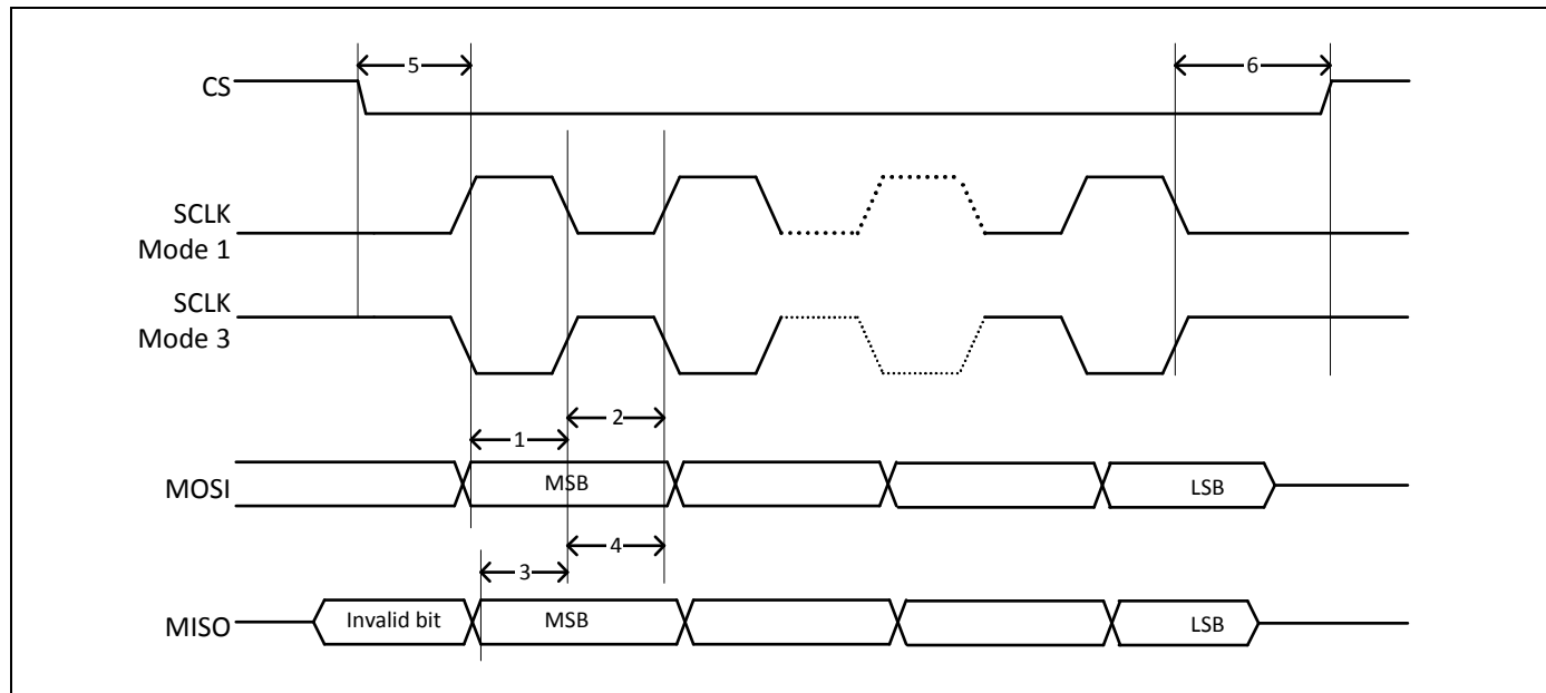
Figure 13. SPI Timing Diagram
