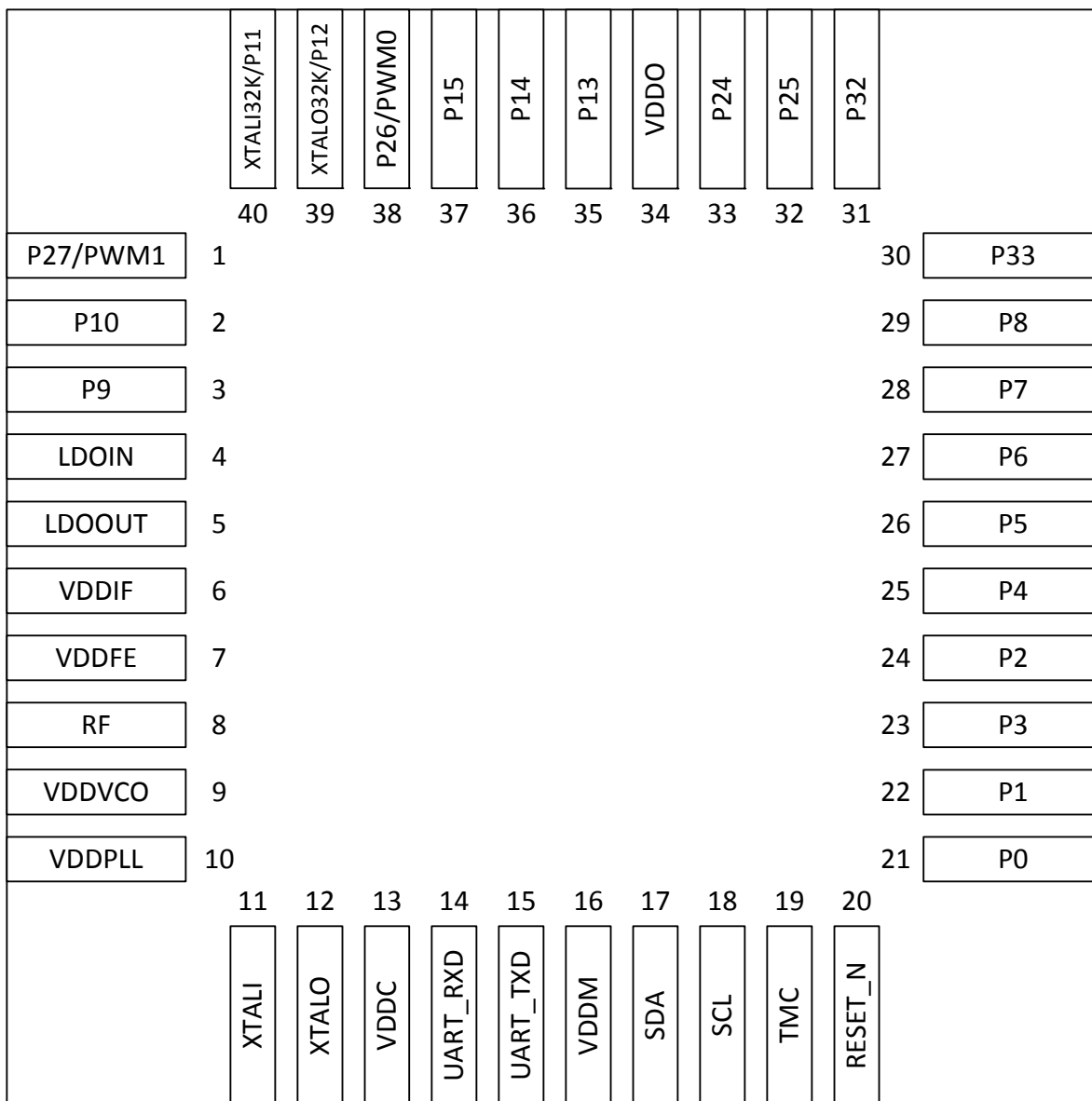
Figure 10. 40-pin QFN Ball Map
