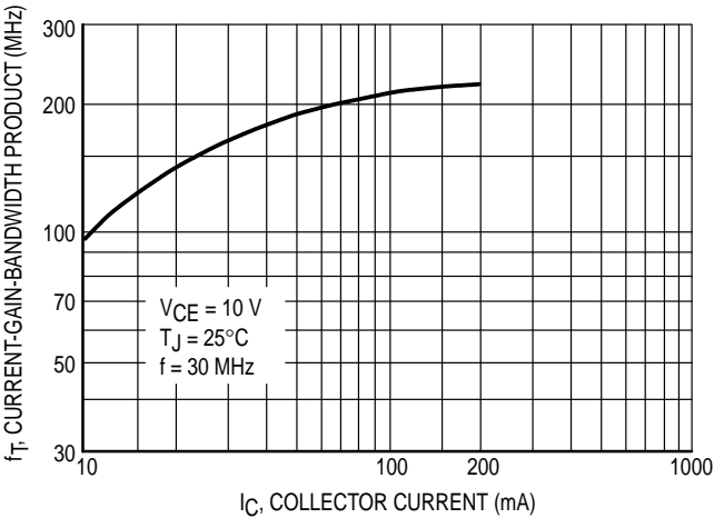
Figure 2. Current-Gain-Bandwidth Product
