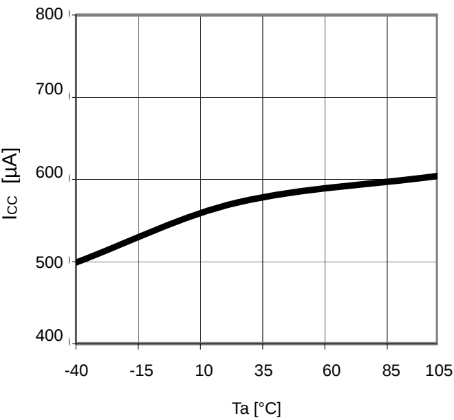
Fig.22 T_a - I_{cc}
