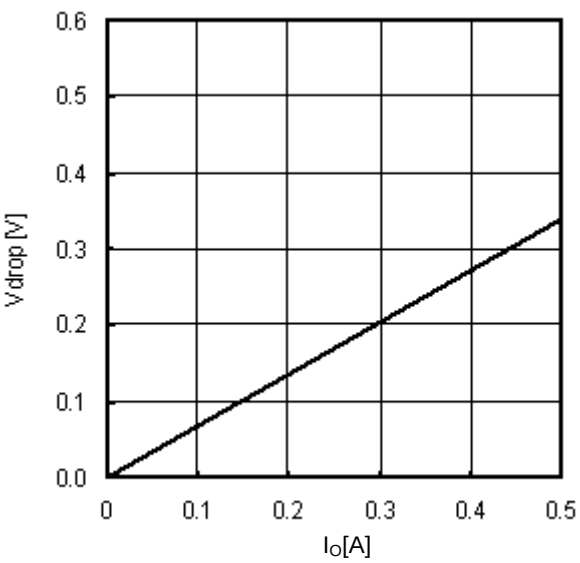
Fig.22 Minimum dropout Voltage 2 ( V_{CC} =2.4V, T_a =25°C)
