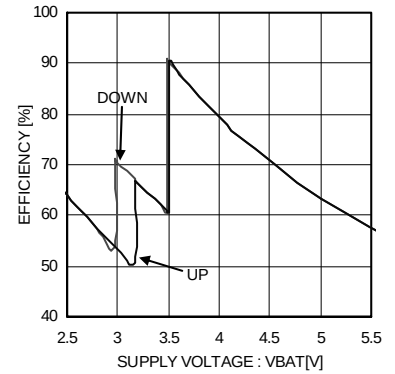
Fig.3 Efficiency Hysteresis (20mA × 4 LEDs)
