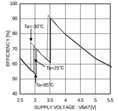
Fig.6 Efficiency (20mA × 4 LEDs)
