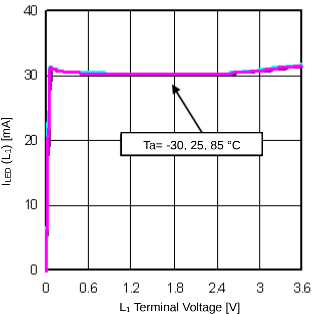
Figure 4. LED Output Current vs LED Pin Voltage ( V_{IN} = 3.6 V, at 32 mA of LED Current)
