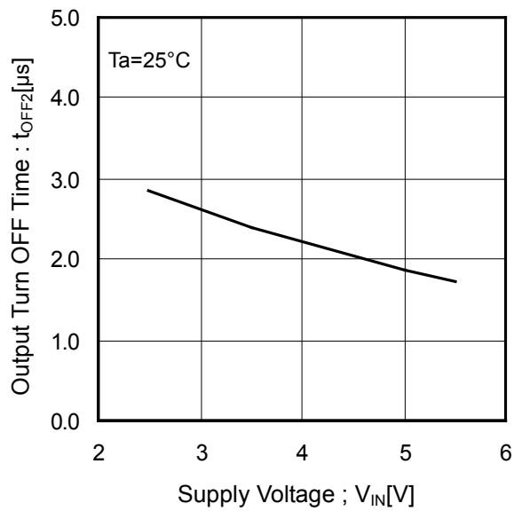
Figure 24. Output Turn OFF Time vs Supply Voltage
