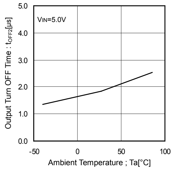
Figure 25. Output Turn OFF Time vs Ambient Temperature
