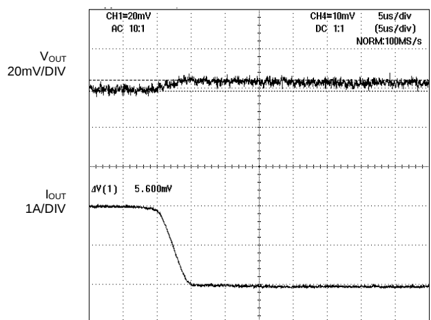
Figure 11. Transient Response (Fall) C OUT =220μF
