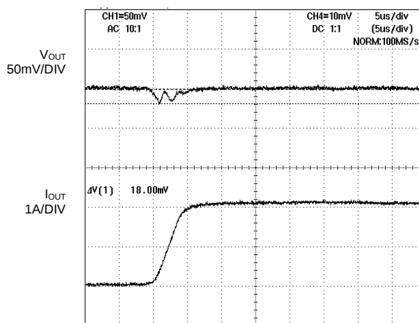
Figure 12. Transient Response (Rise) 47μ MLCC+30mΩ
