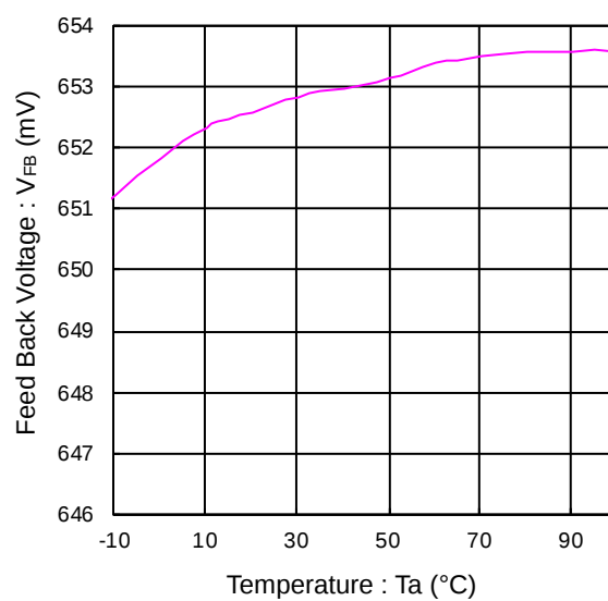
Figure 2. Feed Back Voltage vs Temperature
