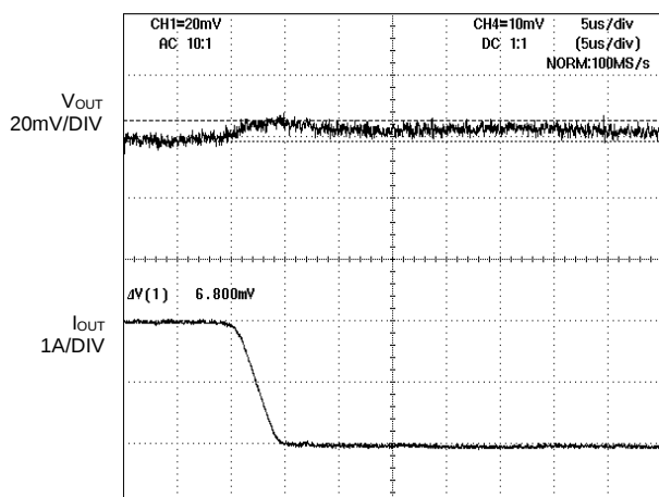
Figure 9. Transient Response (Fall) C OUT =100μF
