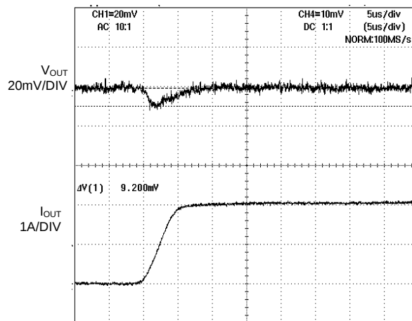
Figure 10. Transient Response (rise) C OUT =220μF
