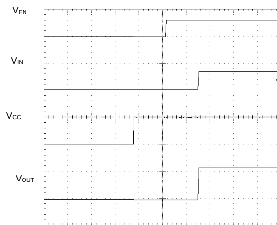
Figure 6. Input Voltage Sequence Final Input Voltage IN
