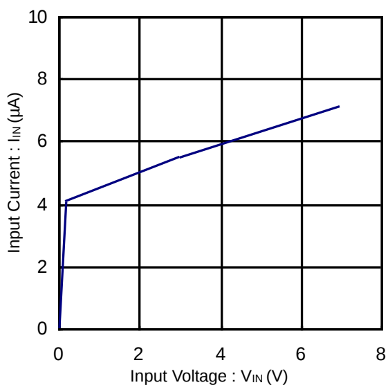
Figure 1. Input Current vs Input Voltage ( T_a=25^{\circ}C )
