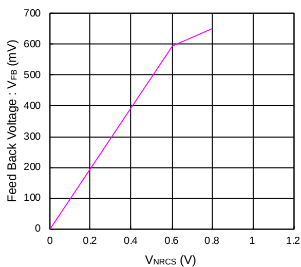
Figure 4. Feed Back Voltage vs V_{NRCS}
