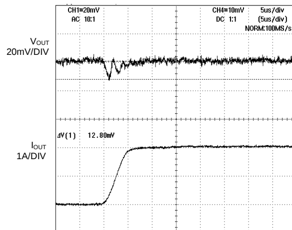
Figure 8. Transient Response (Rise) C_{OUT}=100\mu F
