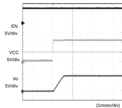
Fig.6 Input sequence 2 C_o=1\mu\text{F}
