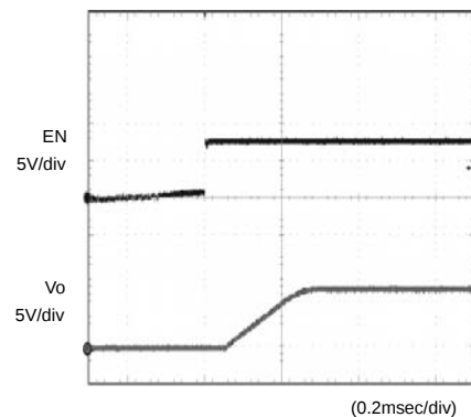
Fig.3 Waveform at output start C_o=1\mu\text{F}
