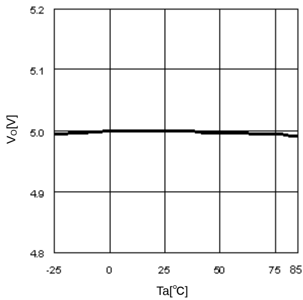
Figure 9. T_a-V_O ( I_O=0mA )
