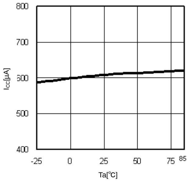
Figure 10. T_a-I_{cc}
