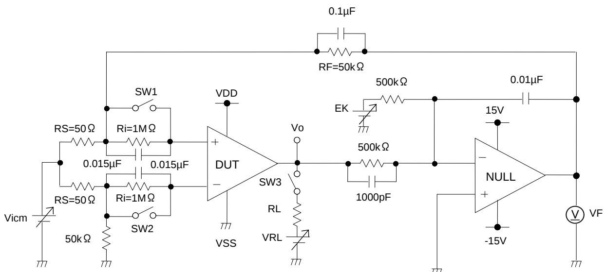
Figure 37. Test circuit 1
