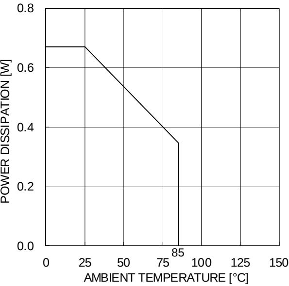
Figure 2. Derating curve
