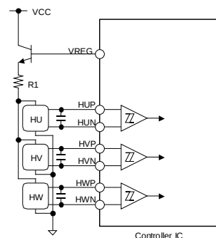
Figure 6. VREG output pin application example
