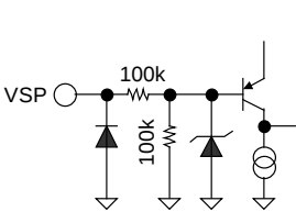
Figure 36. VSP
