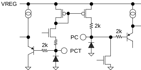
Figure 41. PC, PCT
