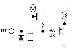
Figure 34. RT
