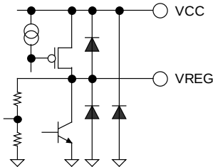
Figure 37. VREG, VCC
