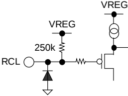
Figure 35. RCL
