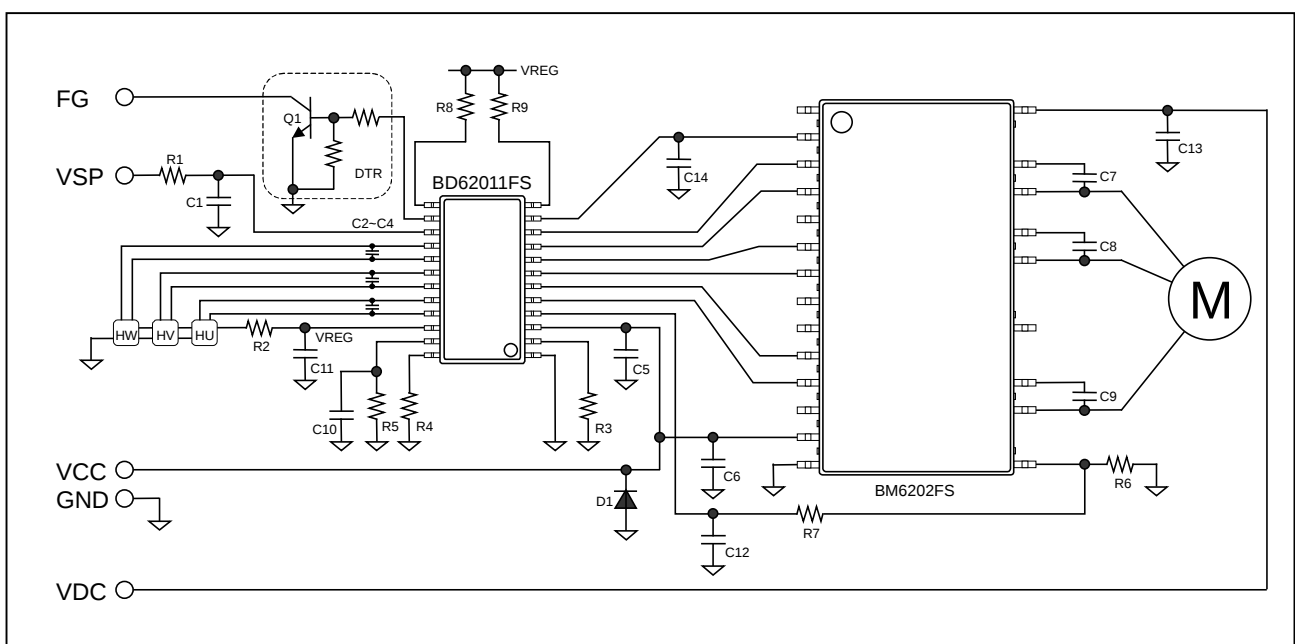
Figure 1. Application circuit example - BD62011FS &amp; BM6202FS
