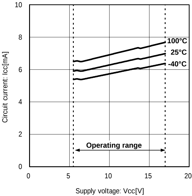
Fig. 3 Circuit current
