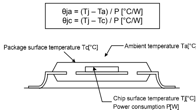
Fig. 53 Thermal resistance
