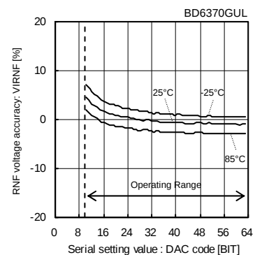
Fig.12 RNF Voltage Accuracy (Const.-Current drive block, R_{DNF}=1.0\Omega , R_L=10\Omega )
