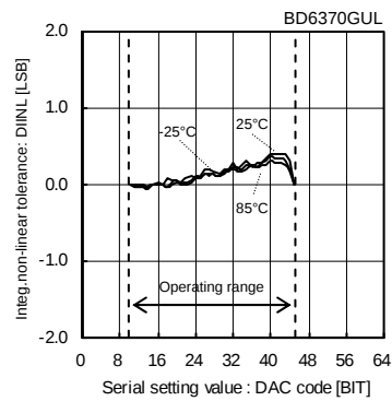
Fig.8 Integral Non-Linear Tolerance (Const.-Current drive block, R_{DNF}=0.5\Omega , R_L=10\Omega )
