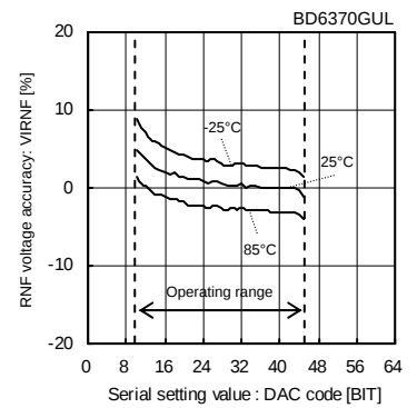
Fig.9 RNF Voltage Accuracy (Const.-Current drive block, R_{DNF}=0.5\Omega , R_L=10\Omega )
