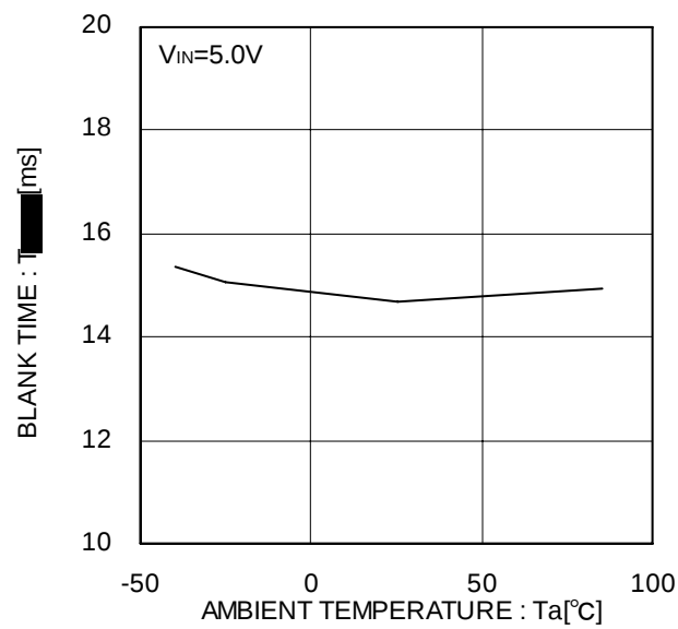
Figure 26. Blanking time
