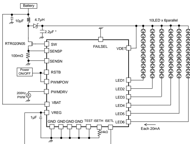
Figure 27. 10 series x 6parallel H current 20mA setting Current driver PWM application
