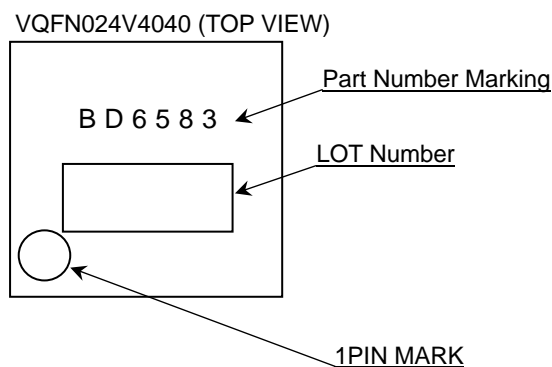
Figure 66. Marking Diagram
