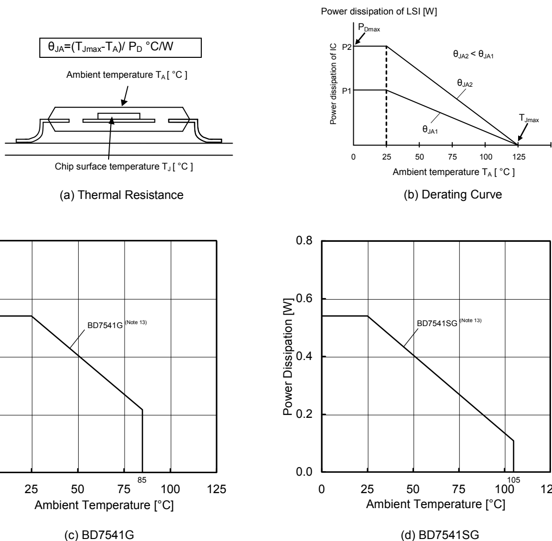
Figure 55. Thermal Resistance and Derating Curve
