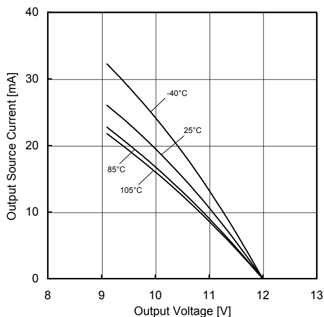
Figure 33. Output Source Current vs Output Voltage (VDD=12V)
