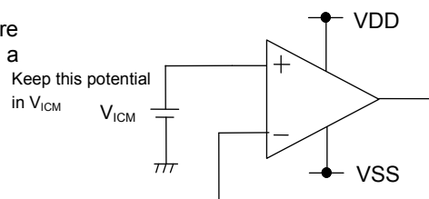
Figure 56. Example of Application Circuit for Unused Op-amp
