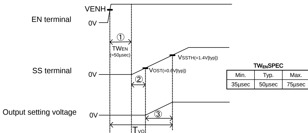
Fig.17 Soft start
