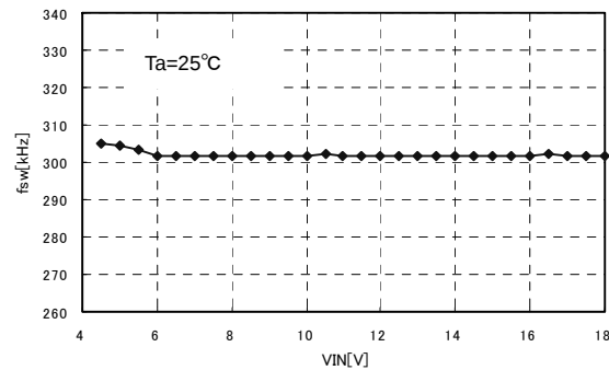
Fig.4 Frequency – VIN characteristic
