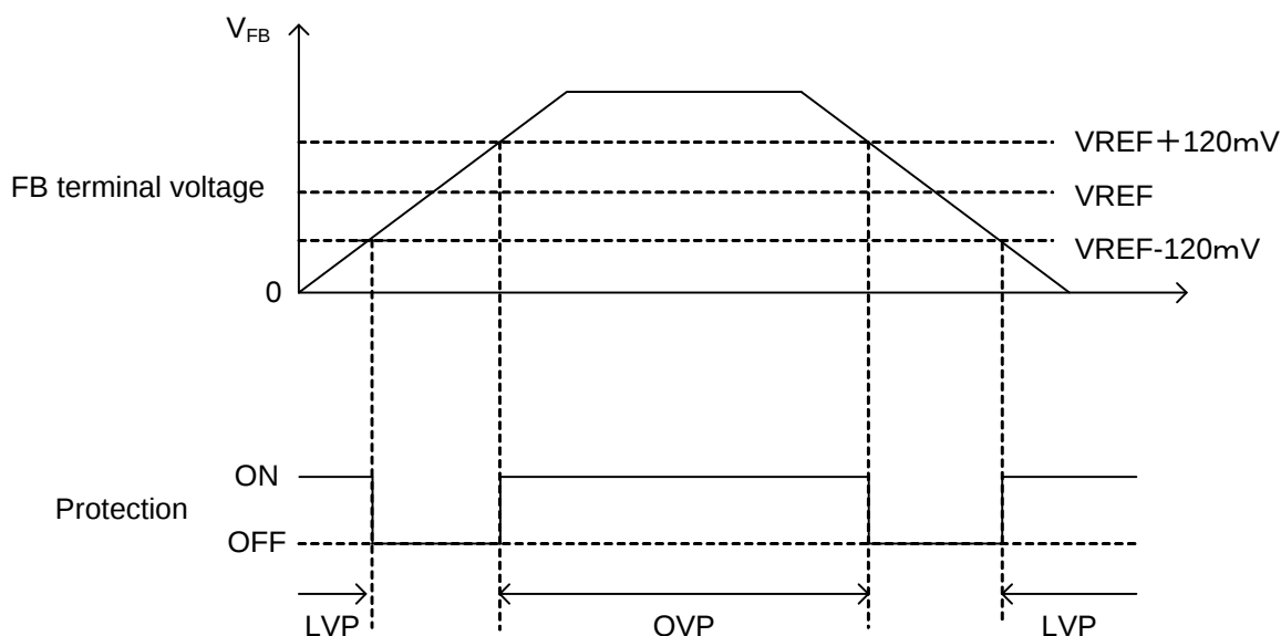
Fig.14 Output voltage error detection range
