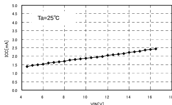
Fig.6 Circuit Current – VIN characteristic
