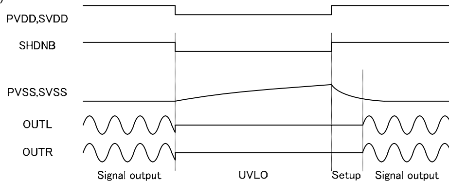
Fig.68 UVLO Operation
