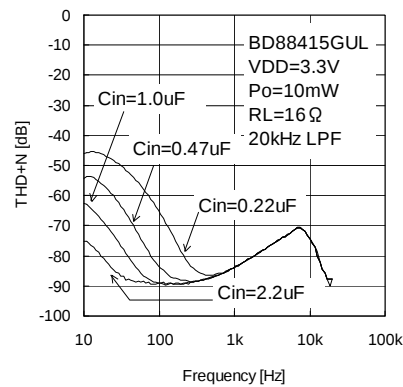
Fig.64 THD+N by the input coupling capacitor (Reference data)
