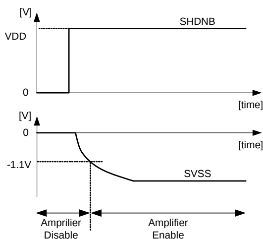
Fig.62 Area of headphone amplifier can operate
