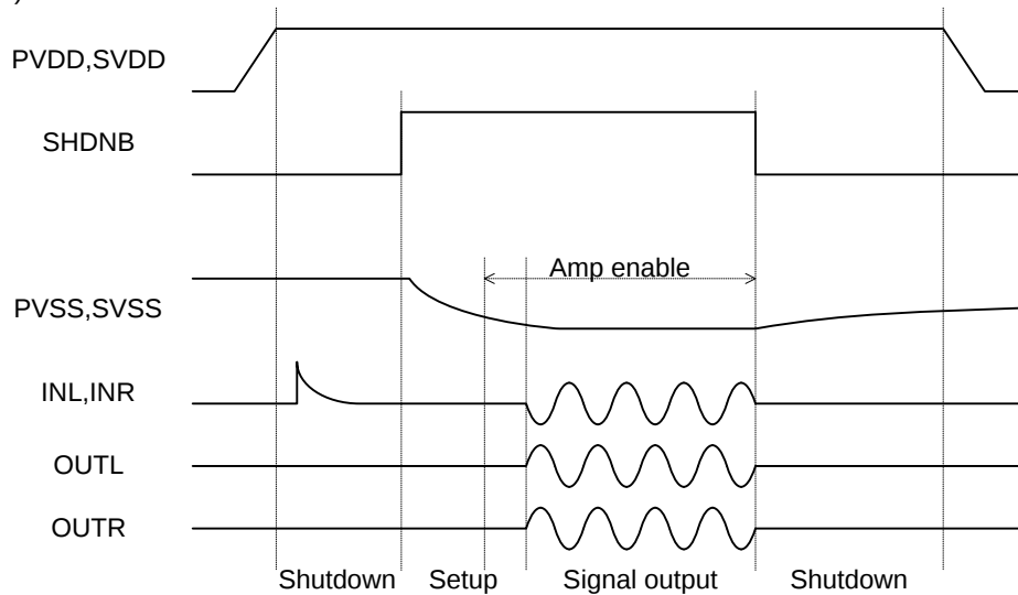
Fig.67 Usually Operation
