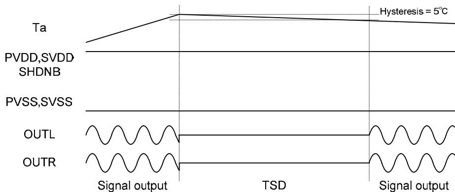
Fig.69 TSD Operation
