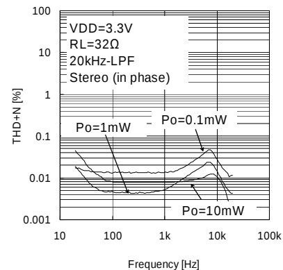
Fig. 46 THD+N vs. Frequency (VDD=3.3V, RL=32\Omega )
