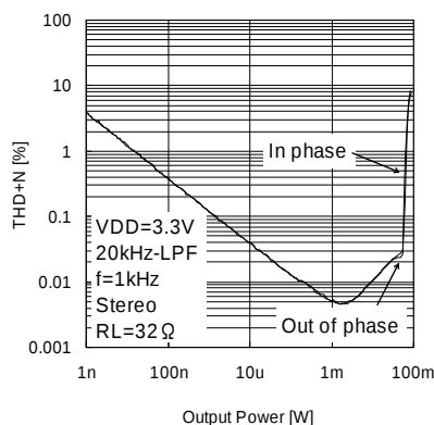
Fig. 44 THD+N vs. Output Power (VDD=3.3V, RL=32\Omega )
