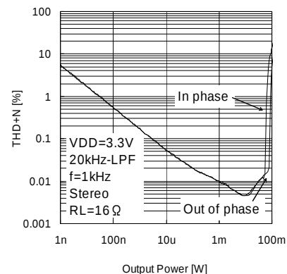
Fig.43 THD+N vs. Output Power (VDD=3.3V, RL=16\Omega )
