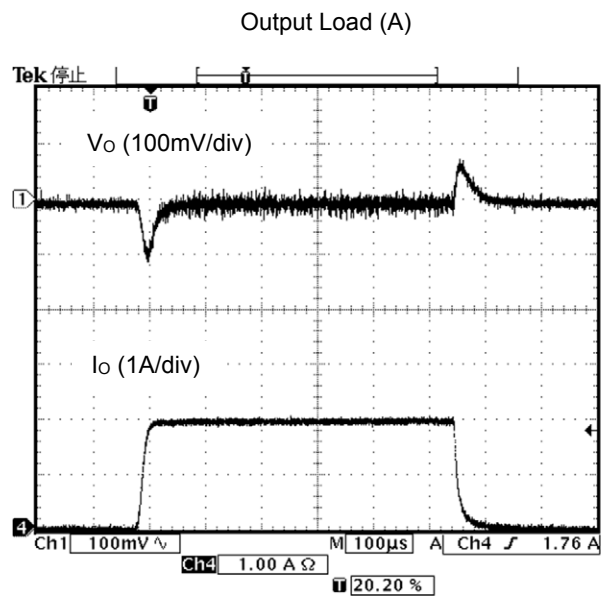
Figure 21. Load Response, I_o=0A \Rightarrow 2A
