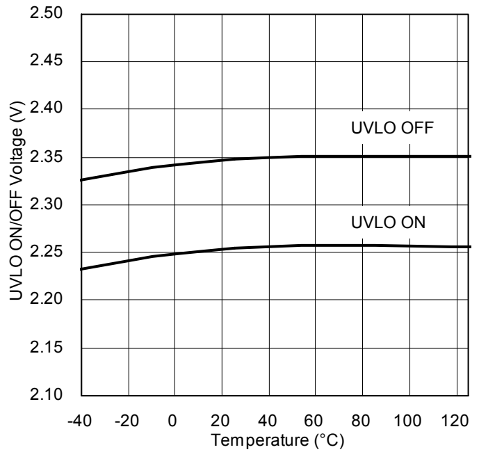
Figure 6. UVLO ON/OFF Voltage vs Temperature
