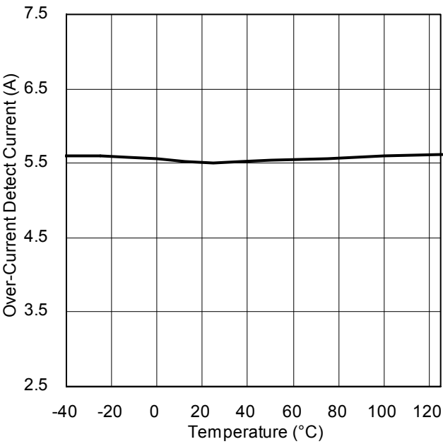
Figure 14. Over-Current Detect Current vs Temperature
