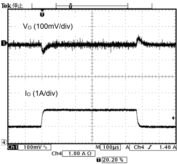
Figure 22. Load Response, I_o=1A \Rightarrow 2A
