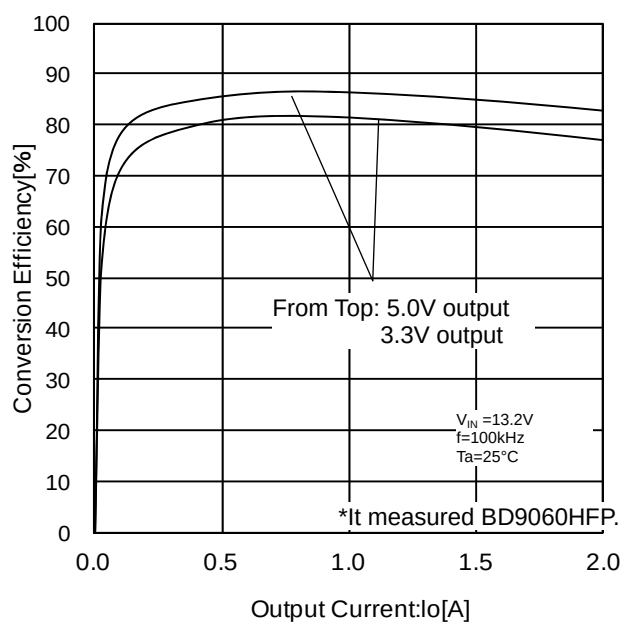
Figure 12. Conversion Efficiency vs Output Current ( f=100kHz )
