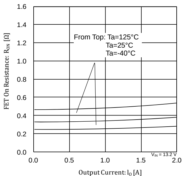
Figure 10. ON Resistance vs Output Current ( V_{IN}=13.2V )
