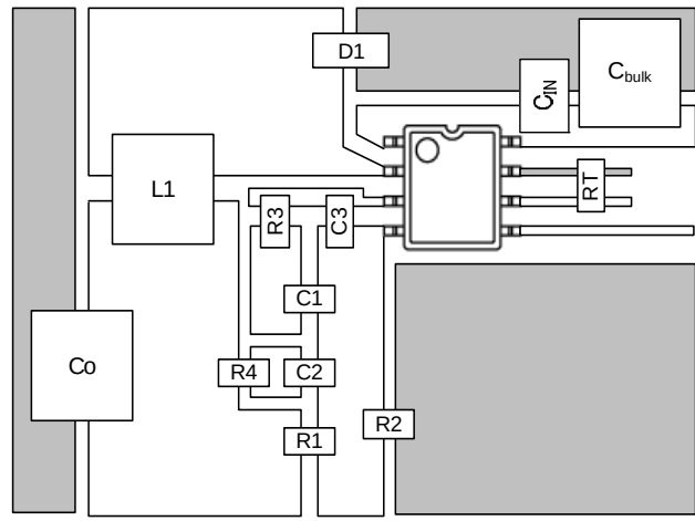
Figure 32. BD9060F-C Reference Layout Pattern
