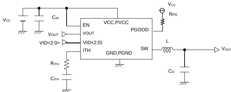
Figure 39. Typical Application
