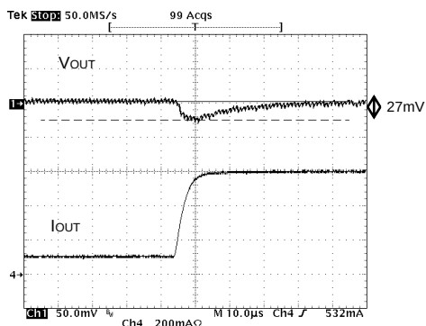
Figure 30. Comparison of Transient Response
