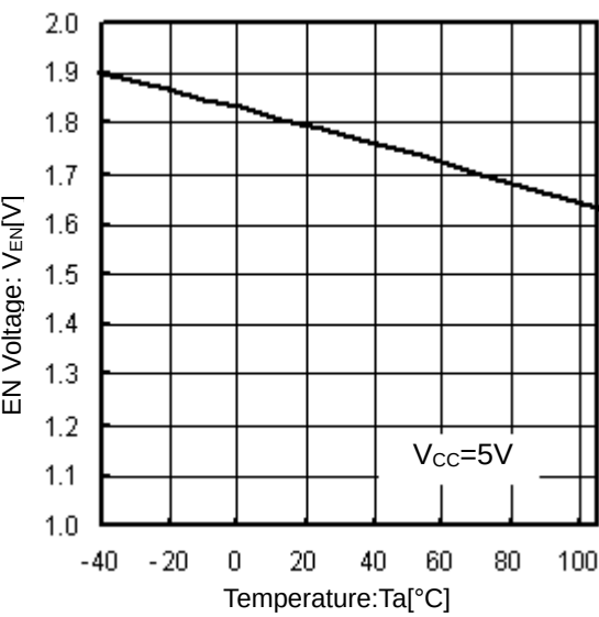
Figure 12. EN Voltage vs Temperature
