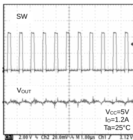
Figure 16. SW Waveform ( I_O=1.2\text{A} )
