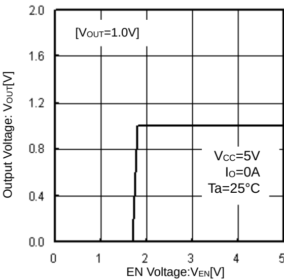
Figure 5. Output Voltage vs EN Voltage
