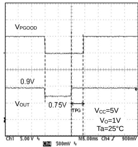
Figure 21. PGOOD Delay
