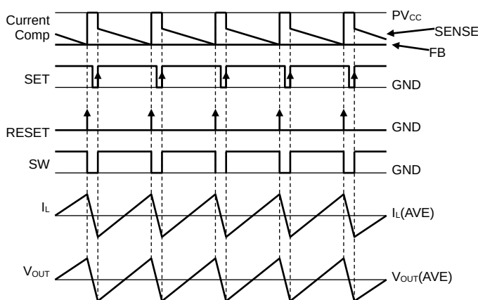
Figure 22. Diagram of Current Mode PWM Control
