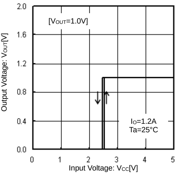
Figure 4. Output Voltage vs Input Voltage
