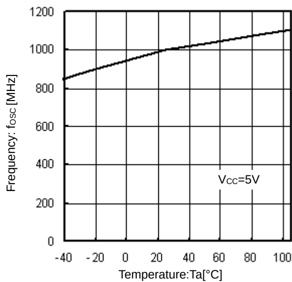
Figure 10. Frequency vs Temperature
