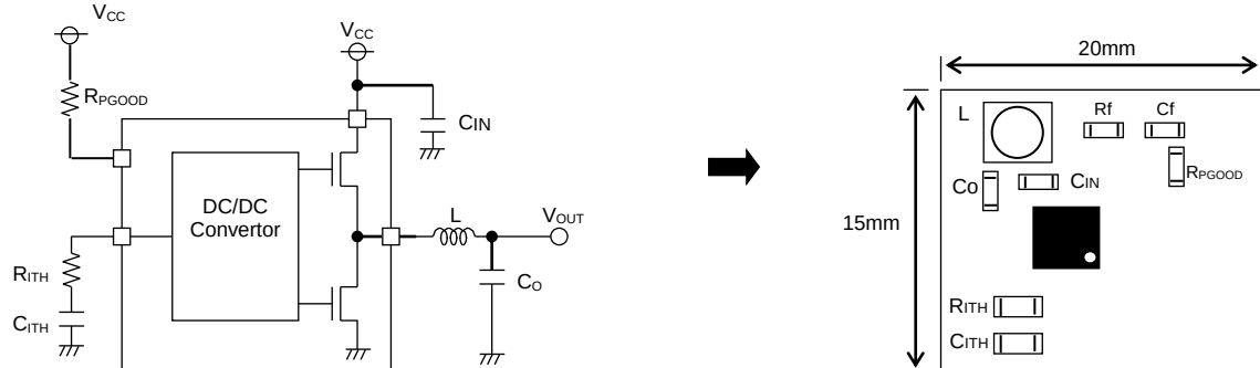
Figure 32. Example of Application
