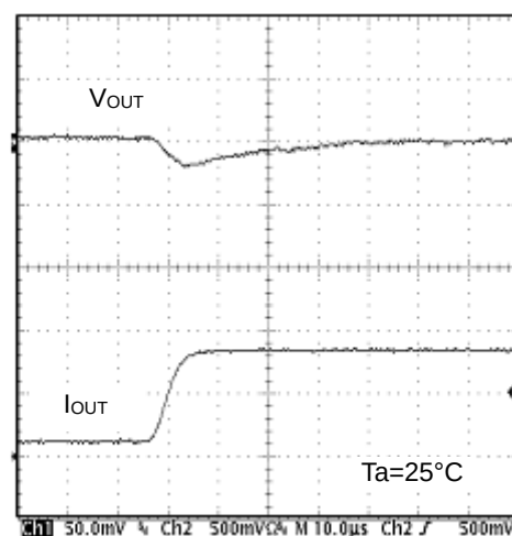
Figure 17. Transient Response ( I_O=125\text{mA} to 850\text{mA} , 2\mu\text{A} )
