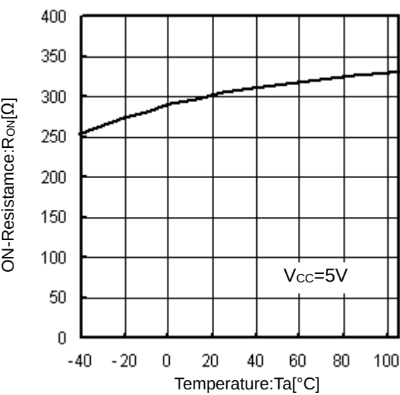
Figure 13. ON-Resistance vs Temperature
