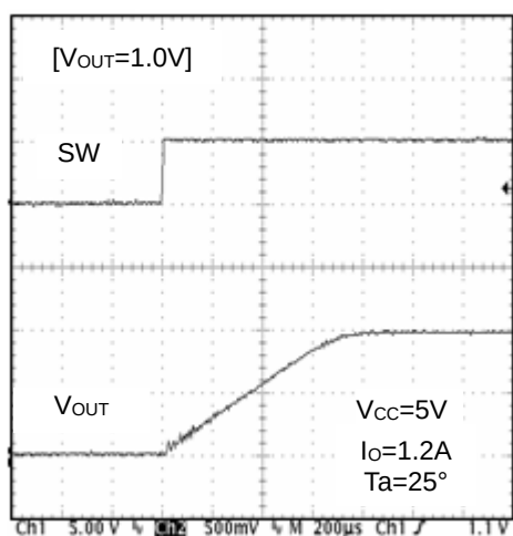
Figure 14. Soft-Start Waveform
