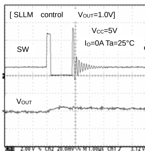
Figure 15. SW Waveform ( I_O=0\text{mA} )
