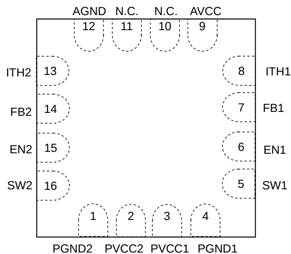
Figure.2 Pin ConFigureuration
