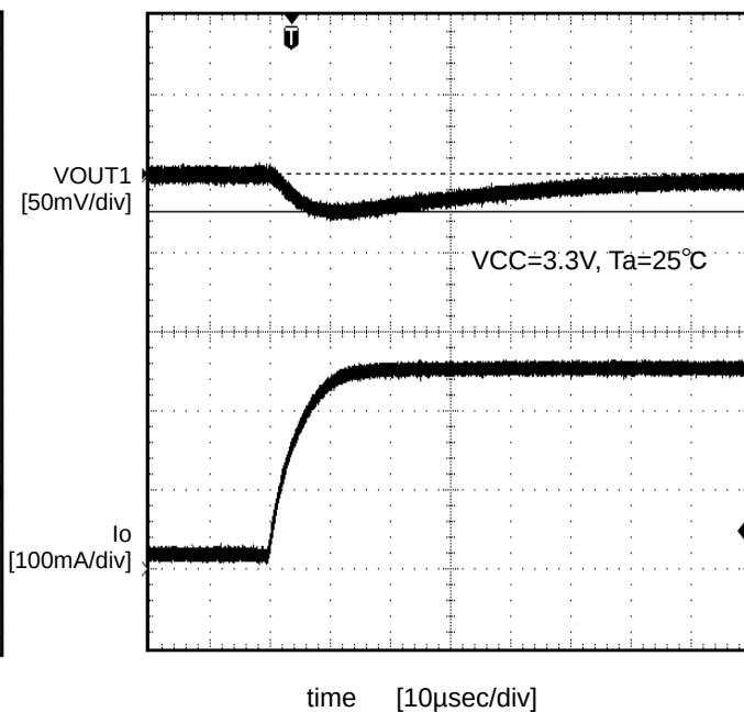
Figure.21 VOUT1 Transient response ( I_o=10mA \rightarrow 0.25A )
