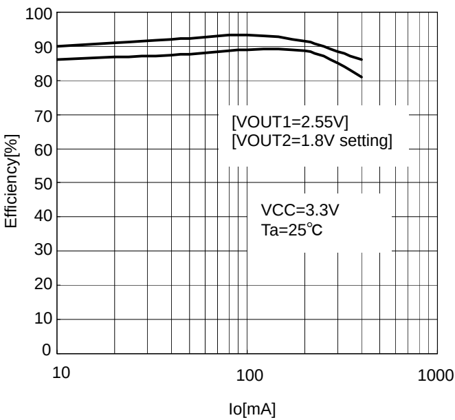
Figure.9 Efficiency
