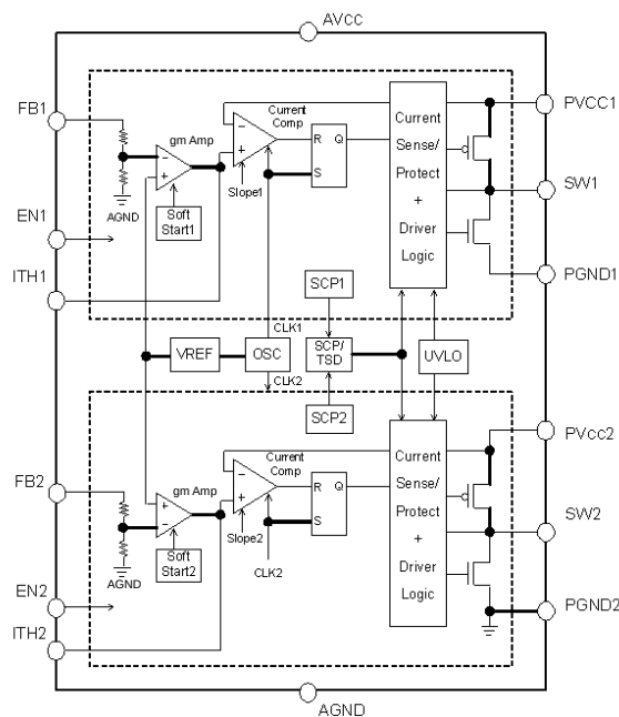
Figure.3 Block Diagram
