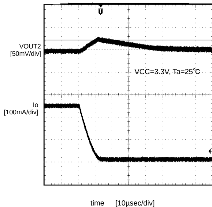
Figure.24 VOUT2 Transient response ( I_o=0.25\text{A}\rightarrow 10\text{mA} )
