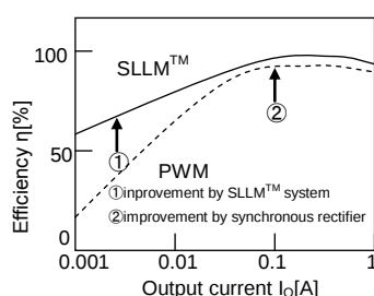
Figure 5. Efficiency
