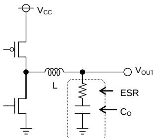
Figure 28. Output capacitor
