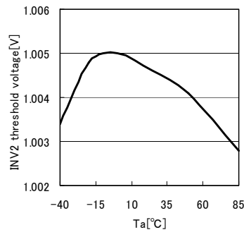
Fig.8 INV2 Threshold Voltage Temperature Feature
