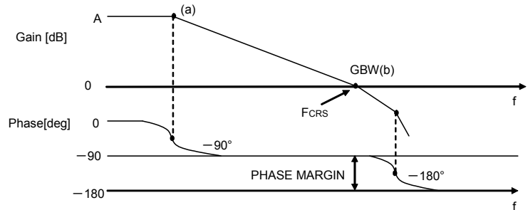
Figure 52. Bode Plot
