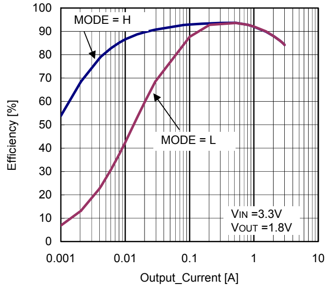
Figure 23. Efficiency vs Load Current ( V_{IN}=3.3V , V_{OUT}=1.8V , L=1.5\mu H )
