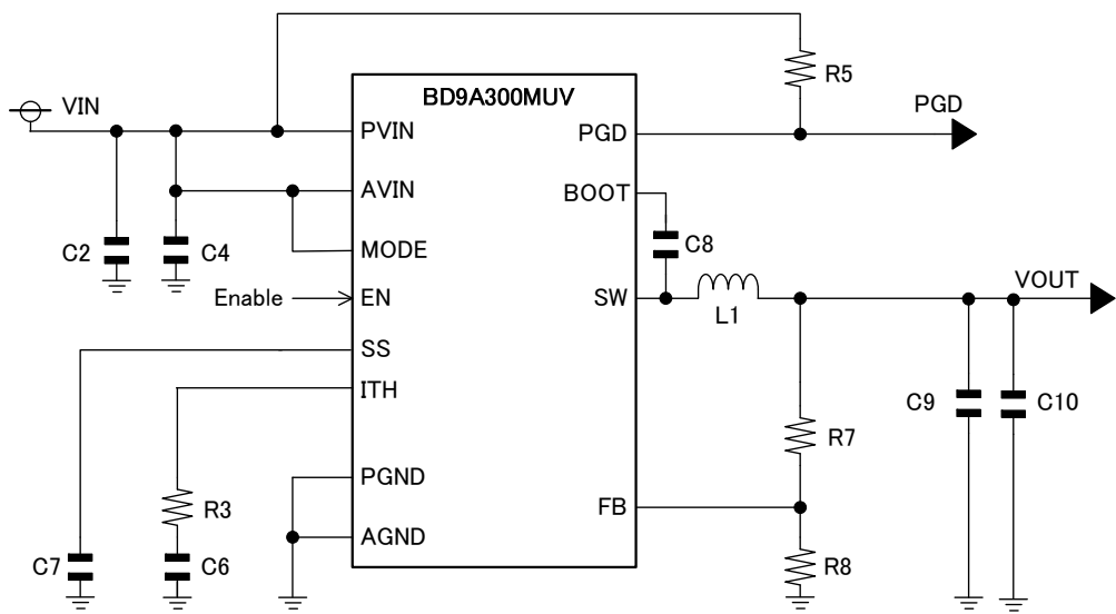
Figure 48. Application Circuit
