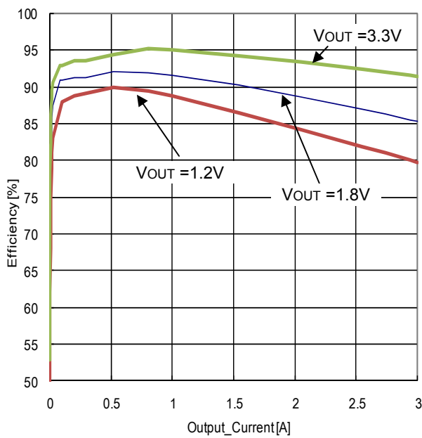
Figure 24. Efficiency vs Load Current ( V_{IN}=5.0V , MODE=5.0V , L=1.5\mu H )
