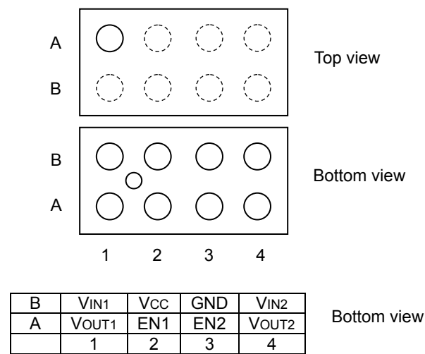
Figure.4 Pin configuration
