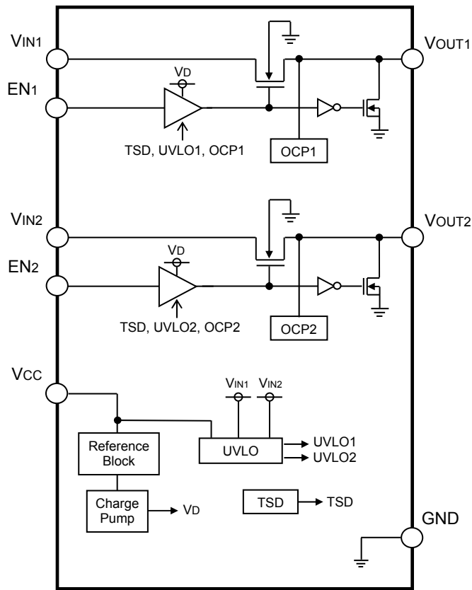
Figure.3 Block diagram
