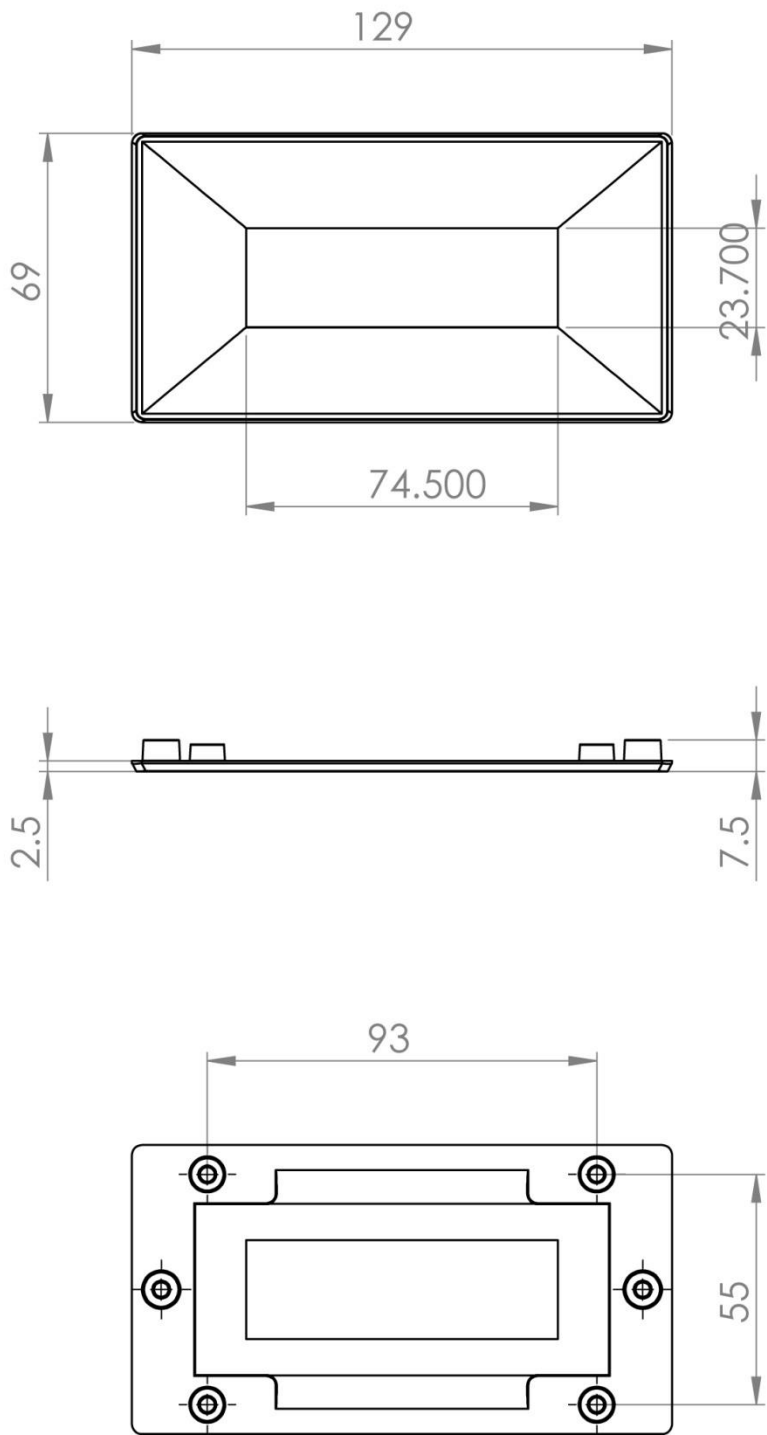
Figure 4: Bez-204A-V1 Dimensions
