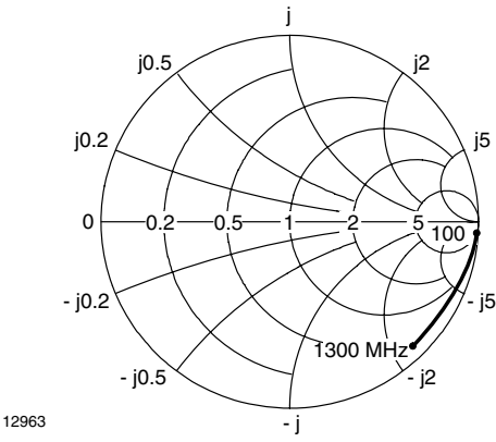
Figure 15. Output Reflection Coefficient
